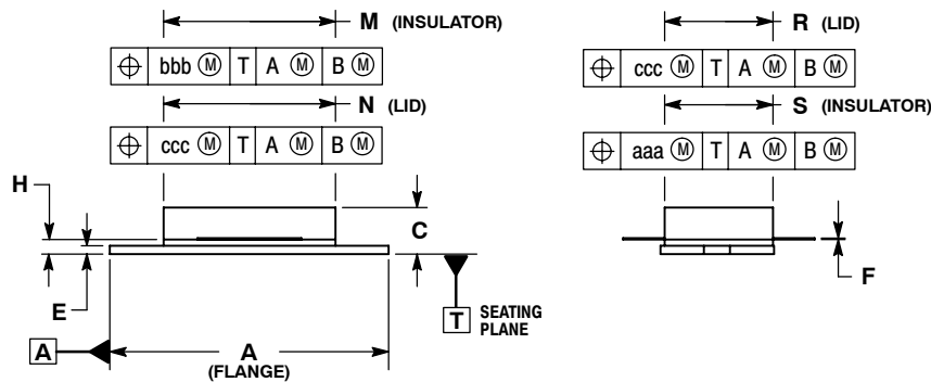
CASE 465B-03 ISSUE E NI-880 MRF6S23140HR3
